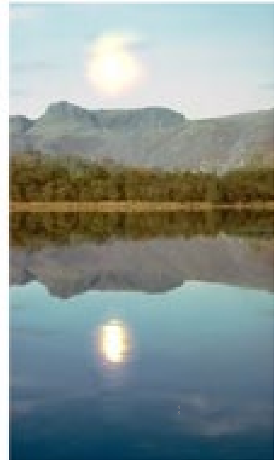
Poisson blending
