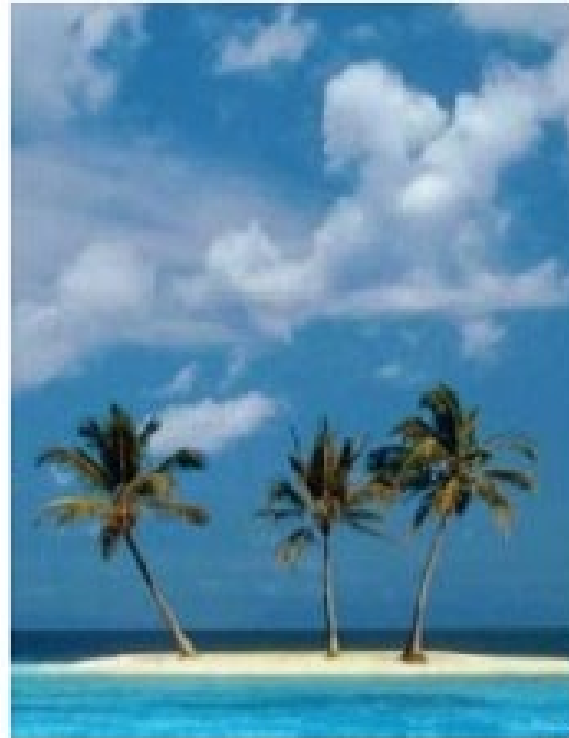
destination
